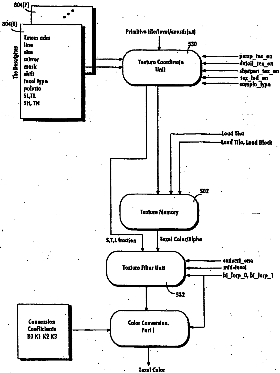
Fig. 23 TEXTURE UNIT EXAMPLE PROCESSES
